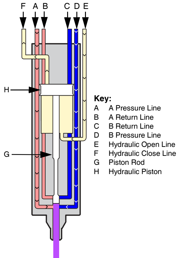
FIG. 15: Dispense
