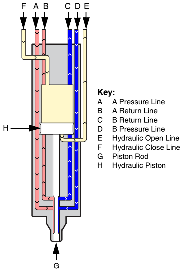
FIG. 14: Circulation
